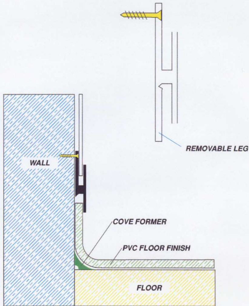
WALL TO FLOOR DETAIL
