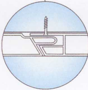
'STRIP CLAD' FLUSH FITTING ABUTMENT DETAIL
