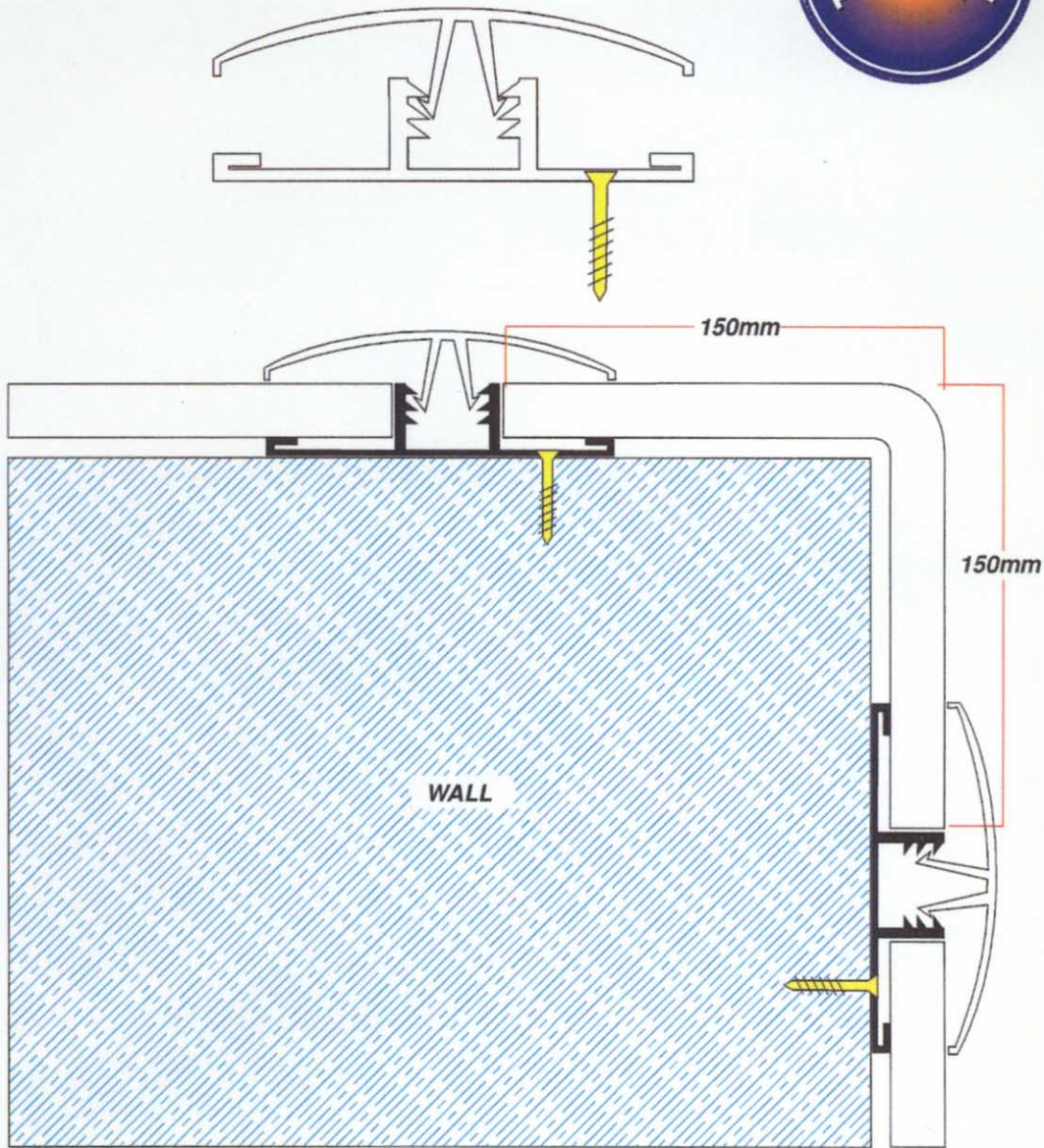
PRE-FORMED EXTERNAL CORNER FIXING
