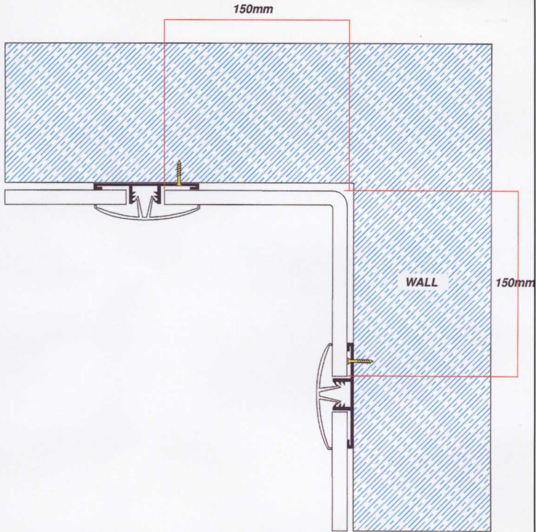
PRE-FORMED INTERNAL CORNER FIXING
