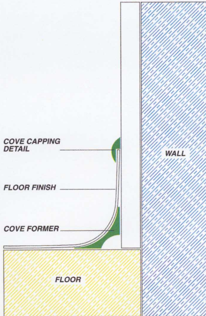
PVC FLOOR WITH COVE FORMER AND CAPPING
