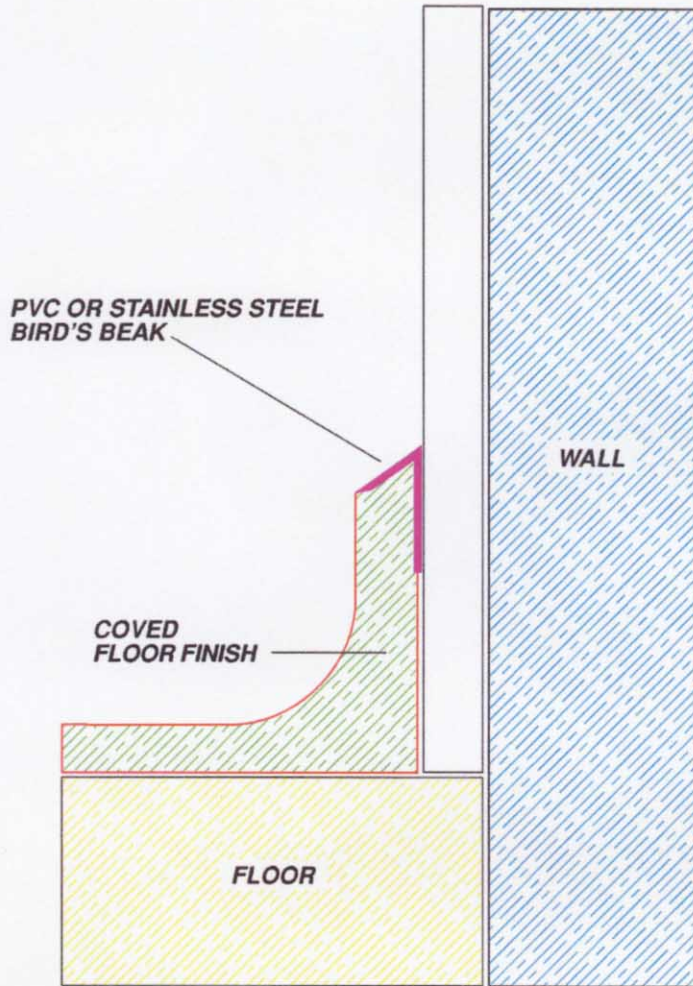
RESIN FLOOR/WALL DETAIL
