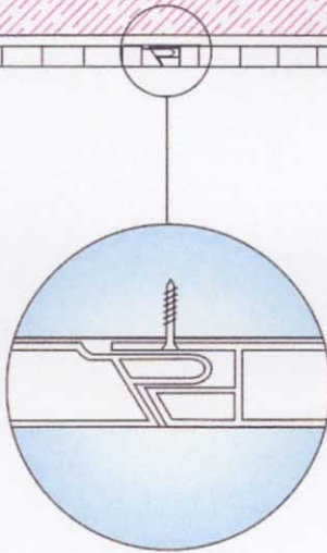
'STRIP CLAD' FLUSH FITTING ABUTMENT DETAIL
