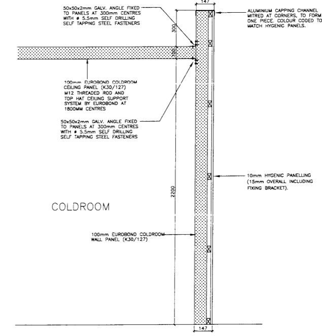
SECTION EE Scale 1:10
