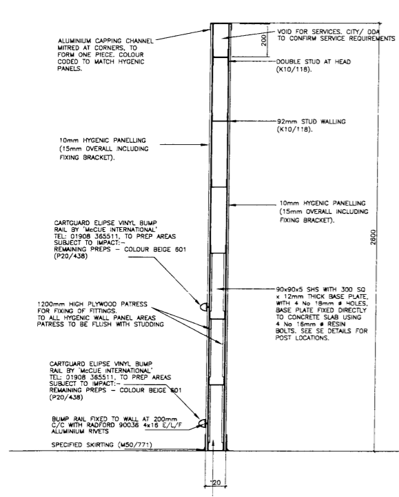
SECTION BB Scale 1:10
